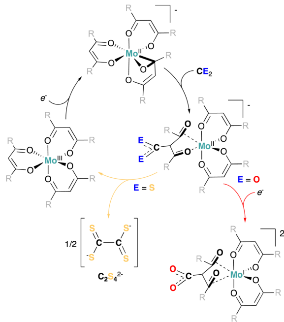
Scheme 3 Generalized mechanistic pattern for the reactivity of [\text{Mo}(\text{Rdiket})_3]^{-1} with \text{CO}_2 (red arrow) vs. \text{CS}_2 (yellow arrow).
