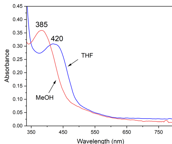
Fig. 8 H-bonding to MeOH causes the RS \rightarrow Fe band of reduced 1 (0.238 mM) to blue-shift relative to its energy in THF.
