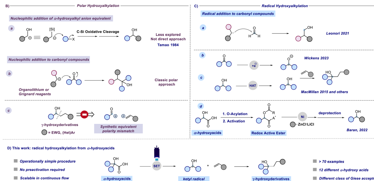
Fig. 1 A) Examples of therapeutic agents containing hydroxyalkyl motifs. Overview of the main approaches for incorporating an \alpha hydroxyalkyl motif in both polar (B) and radical (C) domains. (D) This work unlocks the utilisation of \alpha -hydroxy acids as a synthetic platform for radical hydroxyalkylations.
