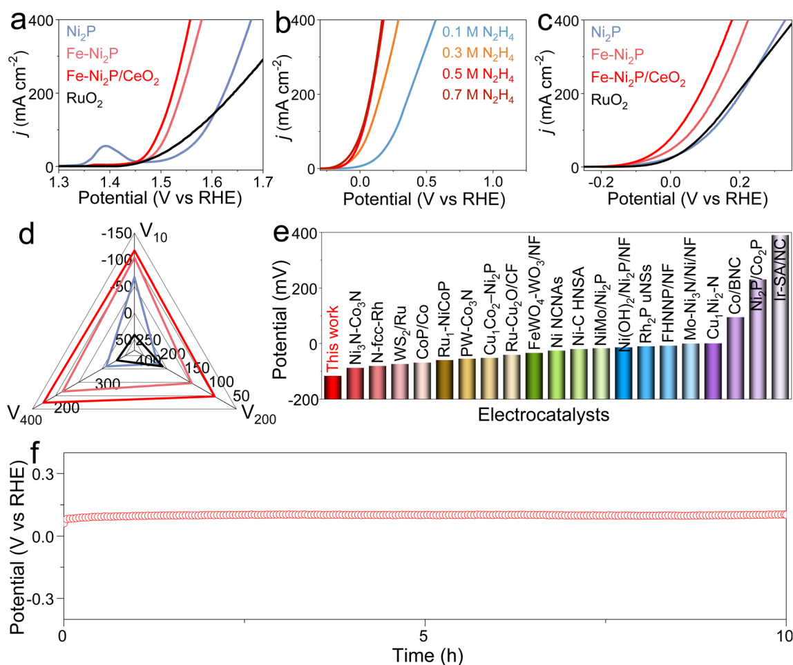
Fig. 4 (a) OER and (c) HzOR polarization curves for Ni 2 P, Fe-Ni 2 P, Fe-Ni 2 P/CeO 2 and RuO 2 . (b) HzOR curves for Fe-Ni 2 P/CeO 2 at various N 2 H 4 concentrations. (d) Potential comparison of the HzOR at 10, 200 and 400 mA cm -2 for Ni 2 P, Fe-Ni 2 P, Fe-Ni 2 P/CeO 2 and RuO 2 . (e) Comparison of the HzOR performances of Fe-Ni 2 P/CeO 2 with recently developed catalysts. (f) Stability test for Fe-Ni 2 P/CeO 2 .
