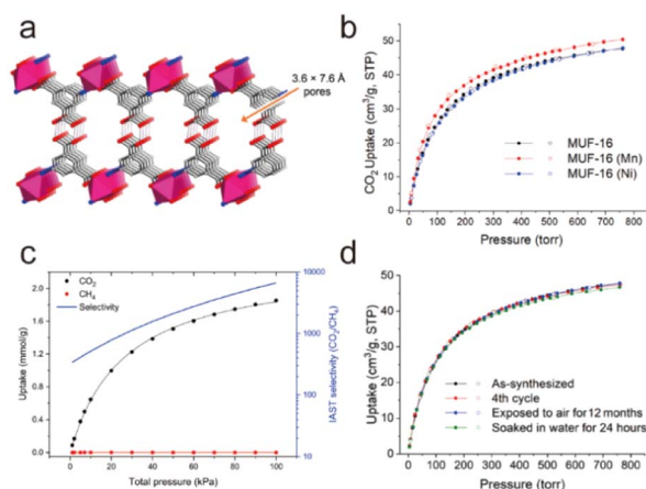
Fig. 44 (a) The structure of MUF-16. (b) The \text{CO}_2 adsorption isotherms of MUF-16s at 293 K. (c) The IAST selectivity of MUF-16 for \text{CO}_2/\text{CH}_4 (50:50) at 293 K. (d) The \text{CO}_2 adsorption isotherms of MUF-16 at 293 K, after 4 consecutive sorption cycles, 12 months of exposure to air with 80% RH, and 24 hours of immersion in water. Reproduced from ref. 265 with permission from Springer Nature, Copyright 2021.
