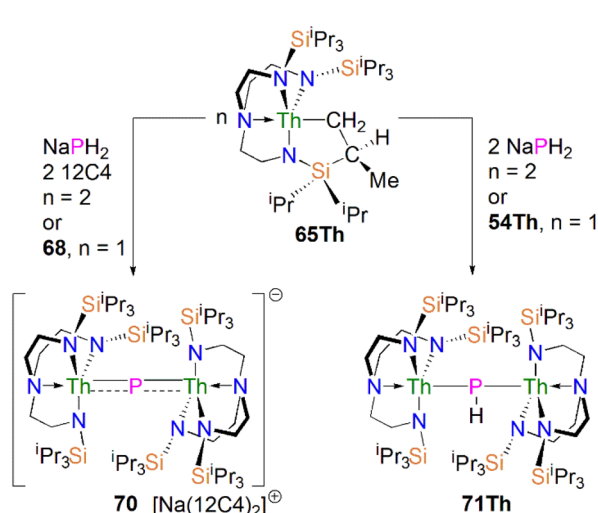
Scheme 23 Synthesis of bridging thorium phosphinidide and phosphido complex 70 and 71Th .
