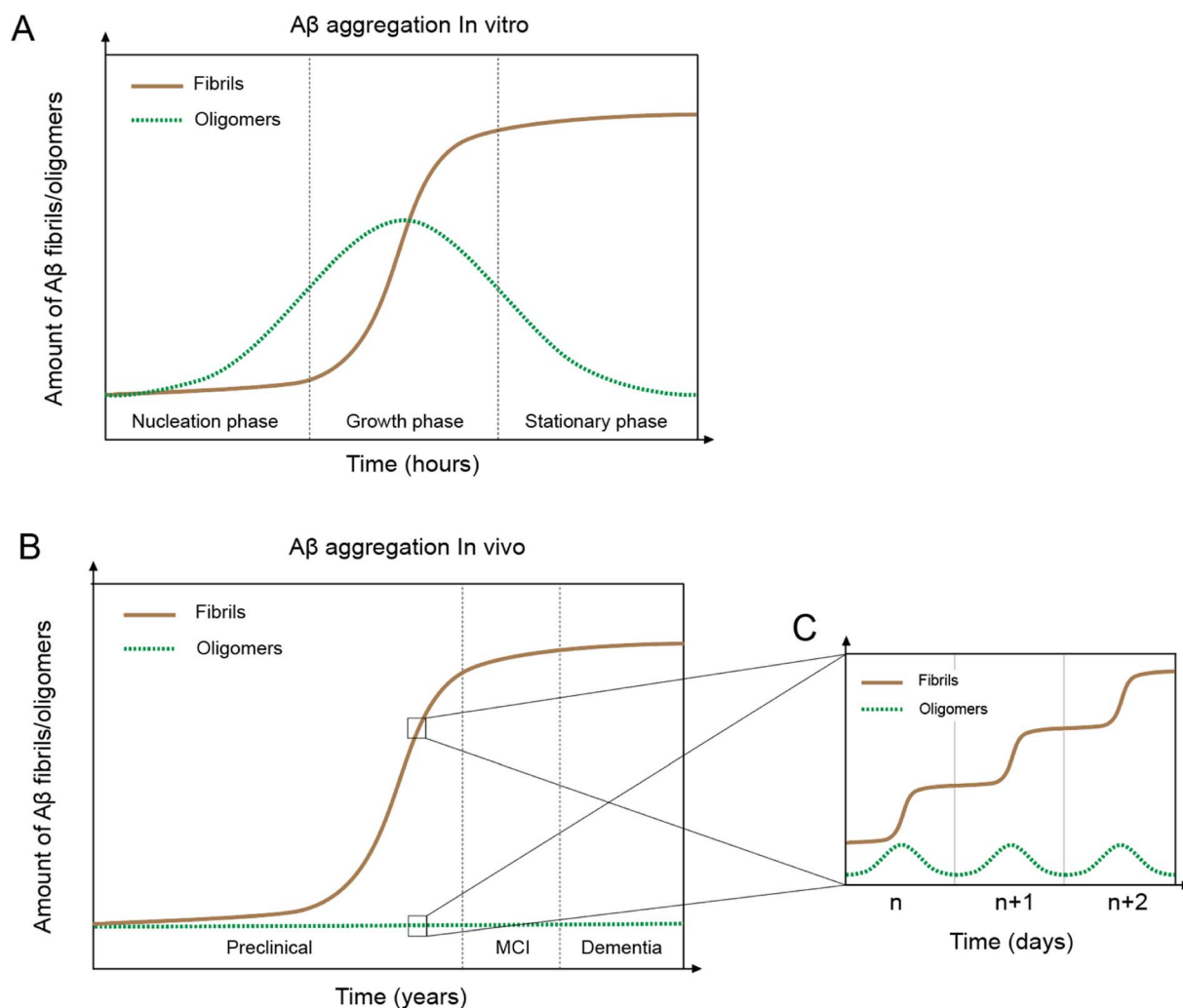
Fig. 2 In vivo and in vitro A\beta aggregation curves. (A) A\beta aggregation in vitro leading to fibril formation (brown line) shows a typical sigmoidal curve with three phases: nucleation, growth, and stationary. Oligomers (green line) first appear in the nucleation phase but disappear towards the end of the aggregation process. (B) A\beta aggregation in vivo displays a similar sigmoidal curve of fibril formation as the in vitro system, but with fundamentally different features. (C) In vivo day-to-day A\beta aggregation shows a sigmoidal curve and oligomer formation.
