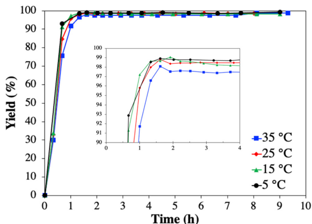
Fig. 6 Progression of yield of modafinil (1) during all four Cr1 experiments conducted at 35, 25, 15, and 5 °C. The inset shows a closer look on 1 yield for the first 4 h to appreciate the small concentration fluctuation prior to achieving steady state.
