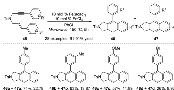
Scheme 15 Synthesis of ADHNs via Fe(II)/Fe(III)-catalyzed and microwave assisted intramolecular DDDA reactions of styrene-ynes.
