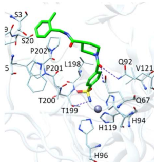
Fig. 136 Chemical structures of compounds 382 and 383 ; their K_i values against hCA-IX and XII along with their docking images.
