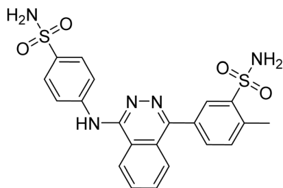
2-Methyl-5-(4-((4-sulfamoylphenyl)amino)phthalazin-1-yl)benzenesulfonamide
