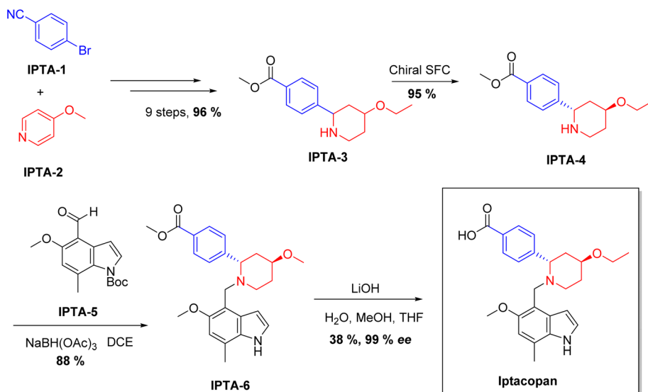
Scheme 16 Synthesis of iptacopan.
