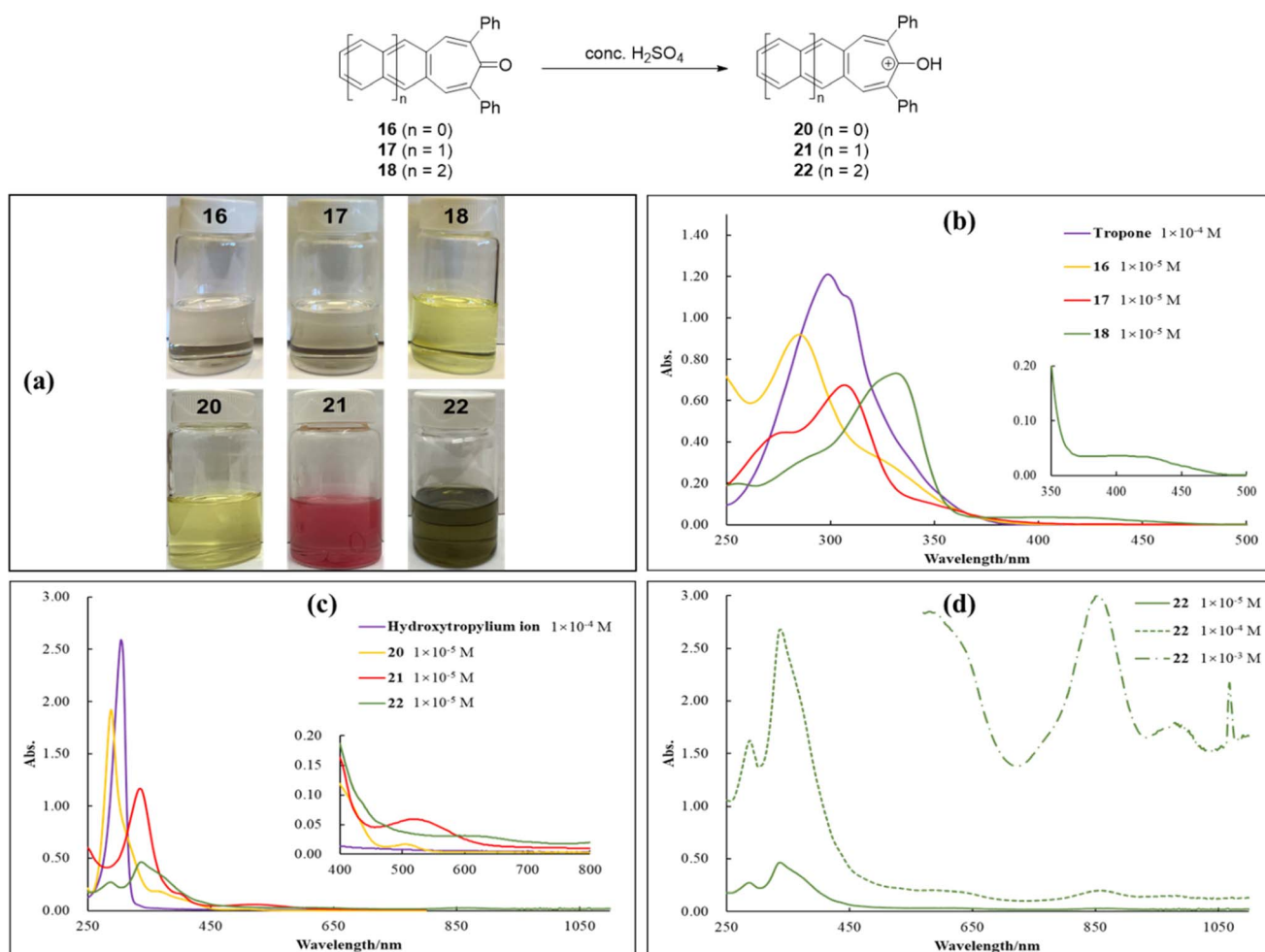
Fig. 5 (a) 1 × 10 −4 M solutions of acenotropones 16–18 in \text{CH}_2\text{Cl}_2 solution and 1 × 10 −4 M solutions of hydroxyacenotropylum ions 20–22 in conc. \text{H}_2\text{SO}_4 ; (b) UV-vis spectra of tropone and acenotropones 16–18 in \text{CH}_2\text{Cl}_2 solution; (c) UV-vis spectra of hydroxyacenotropylum ion and hydroxyacenotropylum ions 20–22 in conc. \text{H}_2\text{SO}_4 ; (d) UV-vis spectra of hydroxyanthracenotropylum ion 22 at several different concentrations in conc. \text{H}_2\text{SO}_4 .
