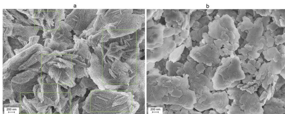
Fig. 4 SEM images of the material obtained by sequential treatment of kaolin from Sulton Uvays (a) and Alyans (b) mines with DMSO, methanol and CTACl (0.1 mol \text{L}^{-1} ).
