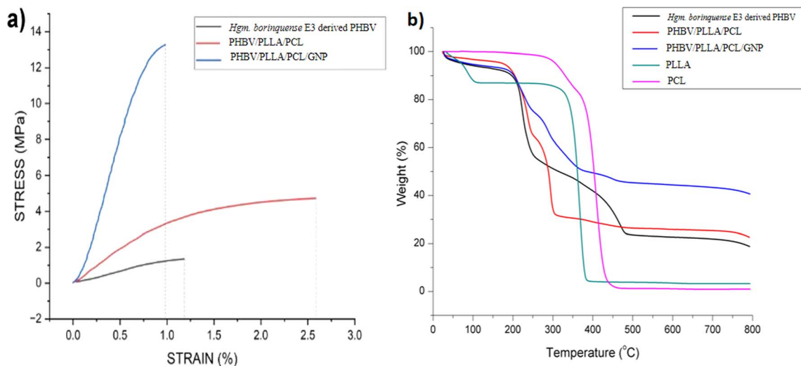
Fig. 4 (a) Stress vs. strain curve of PHBV derived from Haloarchoaeum borinquense E3 and its blend/composite. (b) Thermogravimetric curve of the haloarchaeal PHBV and its blend/composite 45 from 25\text{ }^\circ\text{C} to 800\text{ }^\circ\text{C} .
