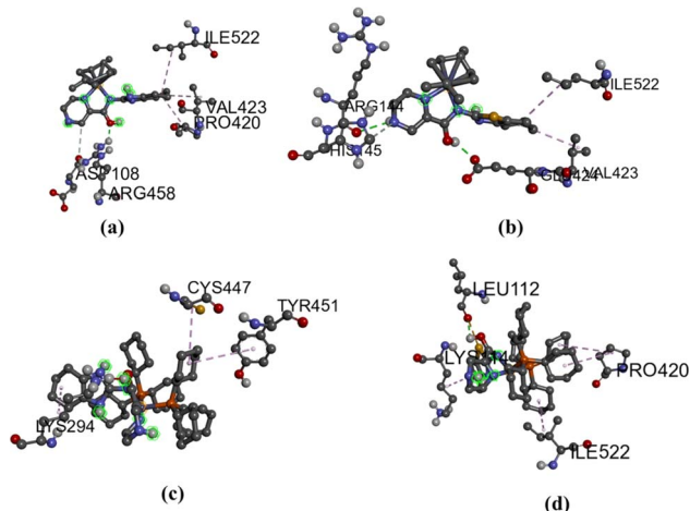
Fig. 6 BSA interactions diagram (scaled ball and stick), (a) Ru1 (b) Ru2 (c) Ru3 and (d) Ru4 with binding scores of -8.0 ( Ru1 ), -7.6 kcal mol ^{-1} ( Ru2 ), 6.6 kcal mol ^{-1} ( Ru3 ) and -6.3 kcal mol ^{-1} ( Ru4 ).
