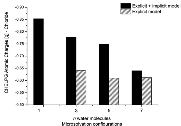
Fig. 7 CHELPG atomic charge calculation (M06-2X/aug-cc-pVDZ) of the nucleofuge ( \text{Cl}^\ominus ) on transition state structure of MS configuration. Filled bar represents explicit + implicit model and striped the explicit model. Transition state for n = 1 (explicit model) and 23 (explicit + implicit model) not found.
