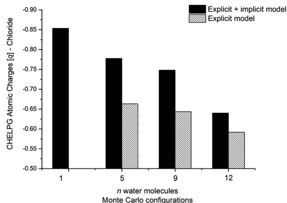
Fig. 4 CHELPG atomic charge calculation (M06-2X/aug-cc-pVDZ) of the nucleofuge ( \text{Cl}^\ominus ) on transition state structures of MC configuration. Filled bar represents explicit + implicit model and striped the explicit model. Transition state for n = 1 (explicit model) not found.
