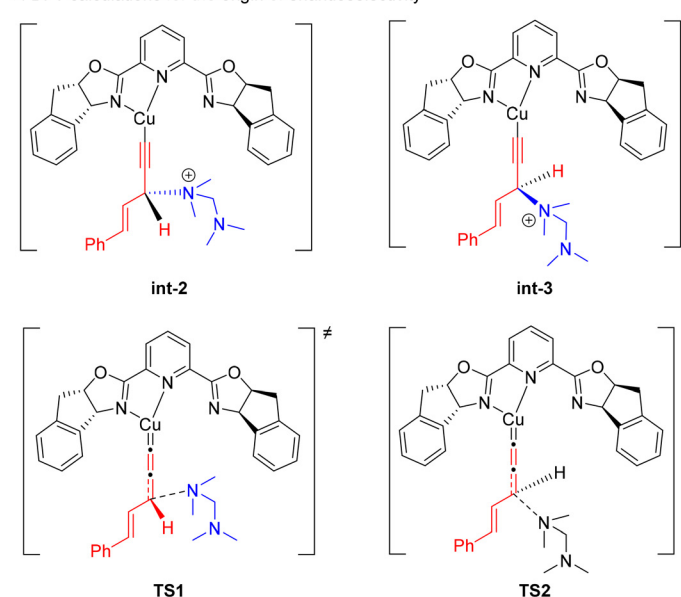
Scheme 4 Preliminary mechanistic studies. BP86/def2tzvp/SMD(methanol)//B3LYP-D3(BJ)/6-31g*/SDD was used for DFT calculations.
