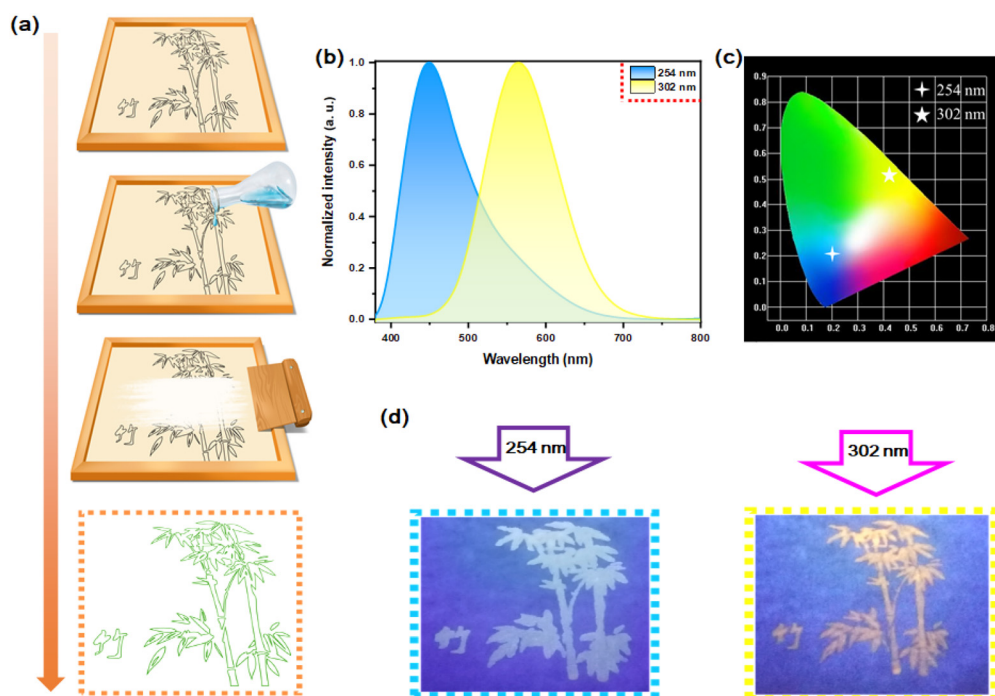
Fig. 11 (a) Schematic diagram of the screen printing process; (b) PL spectra of Rb_2HfCl_6:0.5\%Te^{4+} ( \lambda_{ex} = 254 nm, \lambda_{ex} = 302 nm); (c) CIE coordinates plot diagram of Rb_2HfCl_6:0.5\%Te^{4+} under 254 nm and 302 nm excitation light; and (d) luminescence images of Rb_2HfCl_6:0.5\%Te^{4+} under 254 nm and 302 nm ultraviolet lamps.
