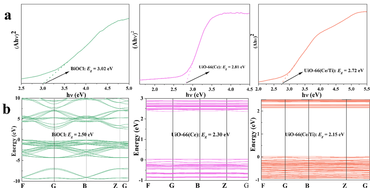
Fig. 3 (a) Plots of (\text{A}h\nu)^2 or (\text{A}h\nu)^2 vs. h\nu for the band gap energy of the samples calculated using the Kubelka–Munk function formula. (b) Band structures of the samples calculated by DFT simulations.
