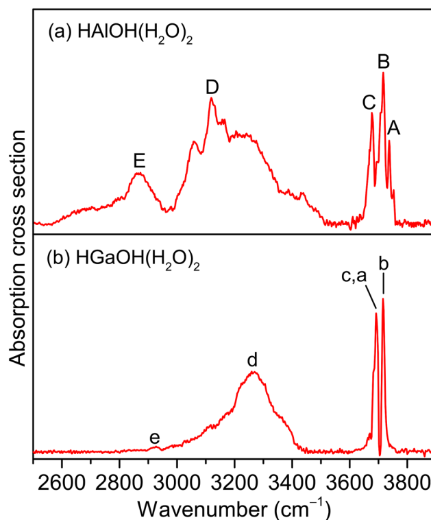
Fig. 1 Experimental IR spectra of neutral HMOH( \text{H}_2\text{O} ) 2 (M = Al and Ga) clusters.
