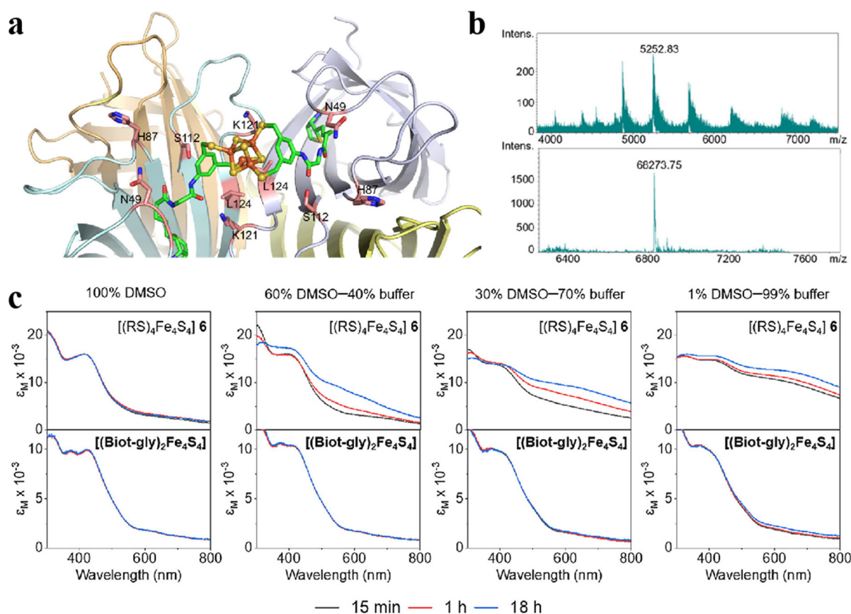
Fig. 10 Artificial Fe–S clusters based on ligand regulation. (a) The structure of Biot-gly ligand-protected Fe 4 S 4 clusters. C: green, O: red, N: blue, Fe: orange, and S: yellow. (b) The mass spectrum of Biot-gly ligand-protected Fe 4 S 4 clusters. (c) The stability of Fe 4 S 4 protected by Biot-gly and RS was compared. Reproduced with permission from ref. 99. Copyright 2023, American Chemical Society.
