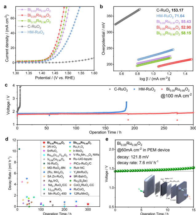
Fig. 3 Electrocatalytic performances of the \text{Bi}_x\text{Ru}_{1-x}\text{O}_2 catalysts towards the OER. (a) Polarization curves in 0.5 M \text{H}_2\text{SO}_4 electrolyte at a scan rate of 5 mV s -1 for the \text{Bi}_x\text{Ru}_{1-x}\text{O}_2 , HM-RuO 2 and C-RuO 2 electrodes. (b) Corresponding Tafel plots of the \text{Bi}_x\text{Ru}_{1-x}\text{O}_2 , HM-RuO 2 and C-RuO 2 electrodes. (c) Chronopotentiometry tests of \text{Bi}_{0.05}\text{Ru}_{0.95}\text{O}_2 , HM-RuO 2 and C-RuO 2 at 100 mA cm -2 in 0.5 M \text{H}_2\text{SO}_4 . (d) Comparison of the operation time (h) and decay rate (mV h -1 ) between the \text{Bi}_{0.05}\text{Ru}_{0.95}\text{O}_2 , \text{Sb}_{0.04}\text{Ru}_{0.96}\text{O}_2 and reported Ir- and Ru-based catalysts at their reported current densities. The star represents stability at a current density of 100 mA cm -2 , the square represents stability at 50 mA cm -2 , and the circle represents stability at 10 mA cm -2 . (e) Chronopotentiometry curve of the PEM electrolyzer at 60 mA cm -2 using \text{Bi}_{0.05}\text{Ru}_{0.95}\text{O}_2 as the anode catalyst in pure water at 80 °C. The inset shows the device diagram.
