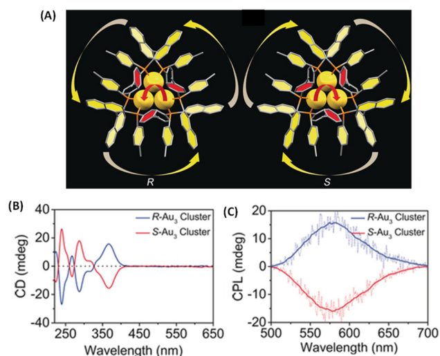
Fig. 7 (A) The overall structures of R/S - Au_3 . Color codes: Au, yellow; P, orange; C, gray. (B) CD spectra of Au_3[(R)\text{-Tol-BINAP}]_3Cl and Au_3[(S)\text{-Tol-BINAP}]_3Cl clusters in DCM. (C) CPL spectra of R - Au_3 and S - Au_3 assemblies in 70% n -hexane. (Reproduced from ref. 45 with permission from John Wiley and Sons, Copyright 2017).
