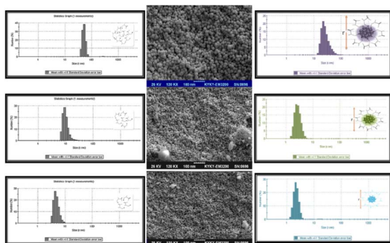
Fig. 9 CuNACs detection at various cyst concentrations as seen using SEM, (Inset): CuNACs size-distribution analysis (1, 100, and 10 \mu\text{M} cyst).
