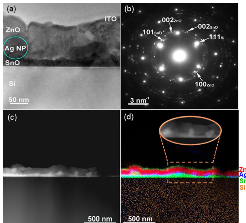
Fig. 8 (a) Conventional transmission electron microscopy (CTEM) image at low magnification of the Si/SnO/Ag NPs/ZnO multilayered structure corresponding to sample Ag@40 and (b) electron diffraction diagram performed on an area from the TEM image shown in (a). (c) HAADF-STEM image of the Si/SnO/Ag NPs/ZnO multilayered structure. (d) Energy dispersive X-ray spectroscopy mapping of the high-angle annular dark-field scanning transmission electron microscopy shown in (c) obtained by overlapping the Si, Ag, Zn, Sn elemental maps. The inset shows a detail of the HAADF-STEM image showing the Ag NPs at the SnO/ZnO interface.
