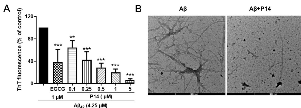
Fig. 4 (A) ThT fluorescence of Aβ incubated with different concentrations of P14. Data are presented as the mean \pm SD, n = 4 , ** P < 0.01 , *** P < 0.001 compared with the Aβ 42 alone group. (B) Representative transmission electron microscopy (TEM) images of Aβ 42 aggregates or Aβ 42 incubated with P14 (50 μM) (24 h) (scale bar = 200 nm).
