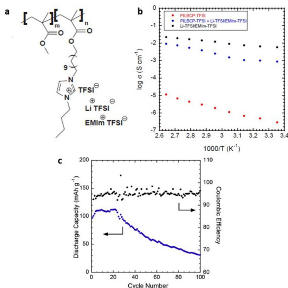
Fig. 29 (a) Schematic representation of the PILBCP-TFSI polymer. (b) Temperature-dependent dry ionic conductivity of PILBCP-TFSI (red), PILBCP-TFSI + Li-TFSI/EMIm-TFSI (blue), and Li-TFSI/EMIm-TFSI (black). (c) Discharge capacity and coulombic efficiency as a function of cycle number and (b) rate is 0.1 \text{ C} . Reproduced from ref. 209 with permission from Elsevier, Copyright [2016].
