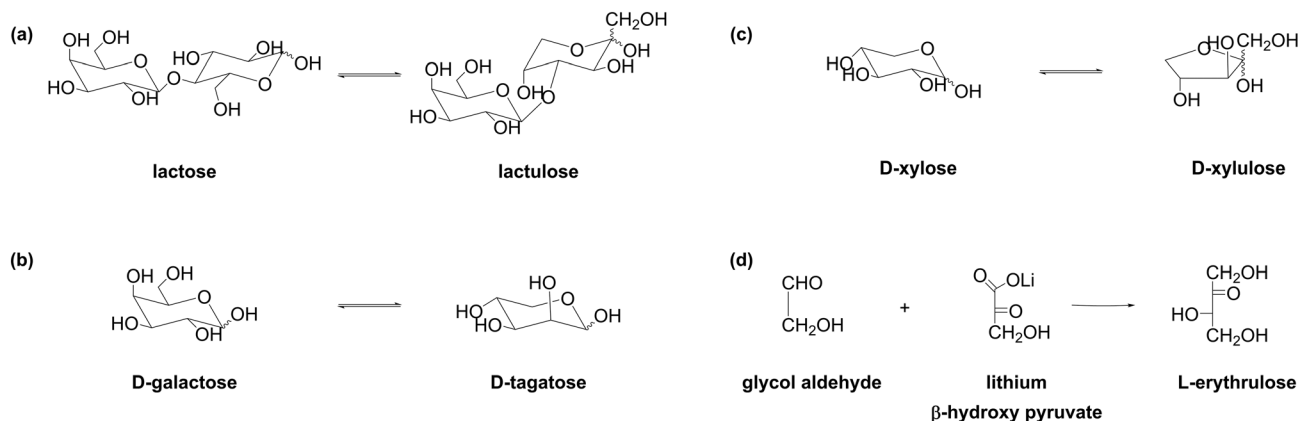
Fig. 6 (a) Isomerization of D-lactose into D-lactulose; (b) isomerization of D-galactose into D-tagatose; (c) isomerization of D-xylose into D-xylulose; (d) conversion of glycolaldehyde and \beta -hydroxy pyruvate into L-erythrulose in the presence of Escherichia coli transketolase.
