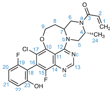
Scheme 1 The chemical structure and numbering of AZD4625.
