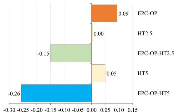
Fig. 8 Results of the oviposition deterrence index (ODI EP ) of the bioactive molecules HT and nanoformulation treatments on S. oryzae females. The index was calculated using the number of wheat seeds with egg plugs relative to the total number of grains, and the number of female weevils. Index values from -1.00 to -0.10 mean repellence, between -0.10 and +0.10 indicate neutrality, while the range +0.10 to +1.00 suggests attraction.
