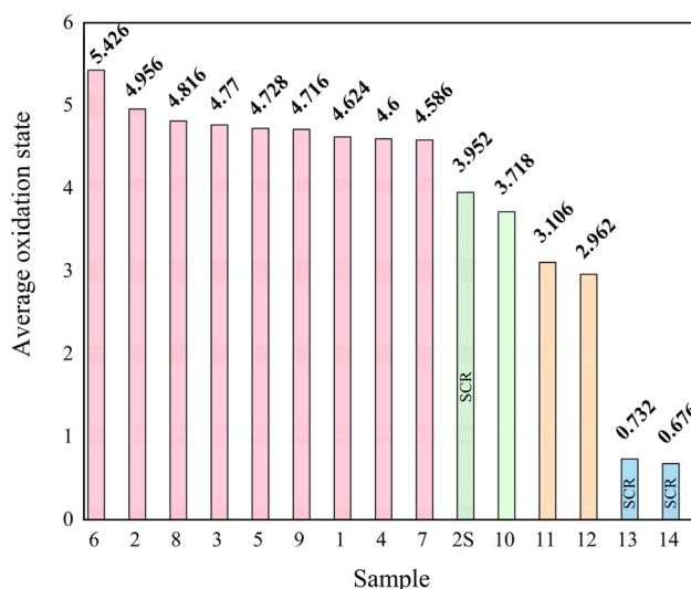
Fig. 6 Average selenium oxidation state for each sample.
