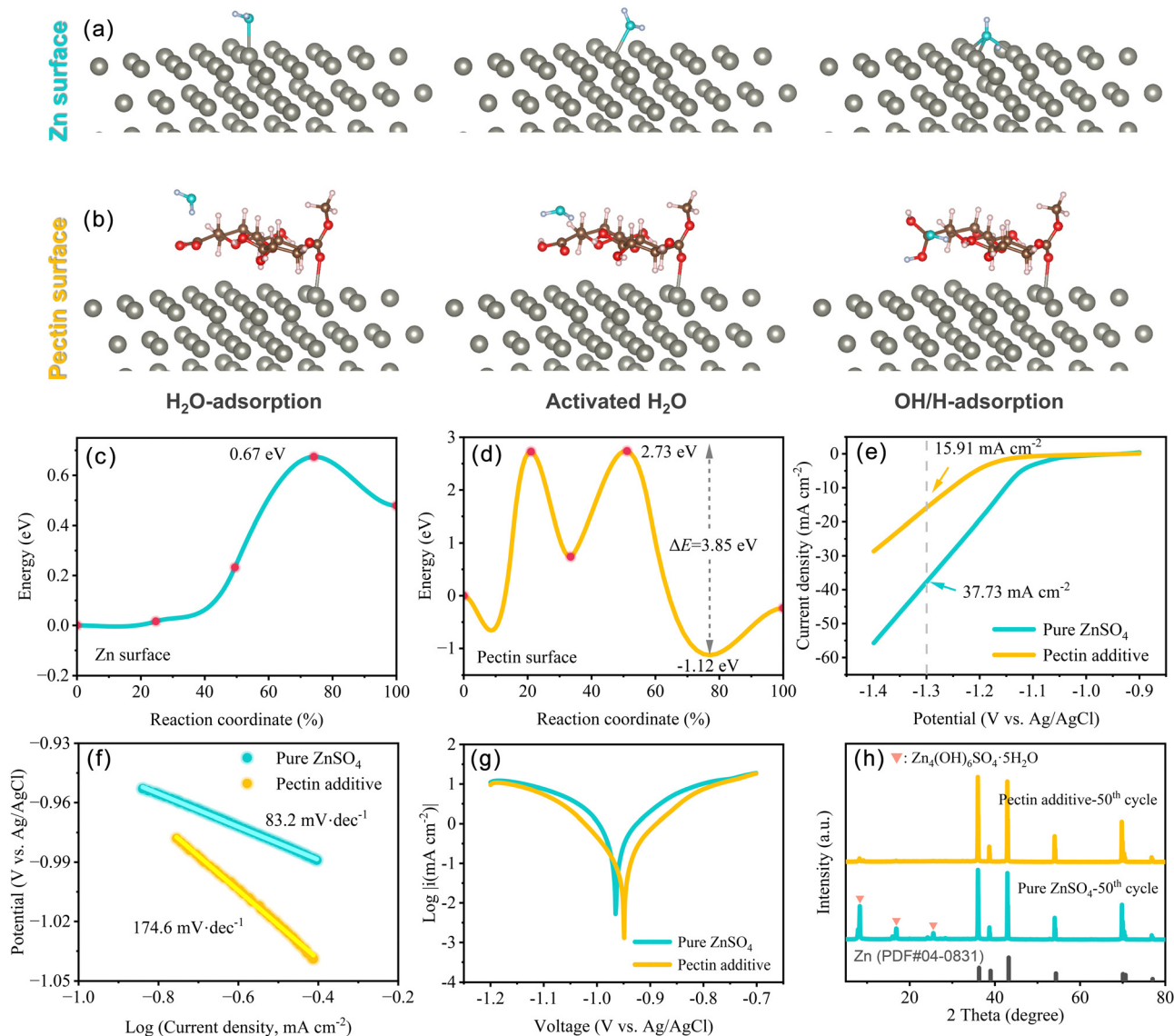
Fig. 3 Inhibition of the side reactions by pectin. DFT calculated adsorption models for H 2 O and activated H 2 O, OH - , and H + on the surface of (a) Zn metal, and (b) pectin molecule. The corresponding dissociation energy barriers of H 2 O in (c) ZnSO 4 -H 2 O and (d) ZnSO 4 -H 2 O-pectin. (e) Hydrogen evolution polarization curves of Zn anodes in pure ZnSO 4 and pectin electrolyte. (f) The corresponding Tafel slope curves. (g) Corrosion curves of Zn anodes in pure ZnSO 4 and pectin electrolyte. (h) XRD patterns of Zn anodes in pure ZnSO 4 and pectin electrolyte after 50 cycles.
