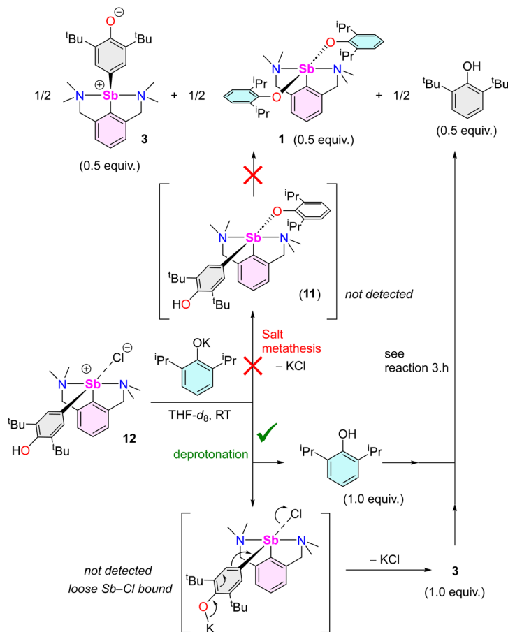
Scheme 5 Reaction of [\{\text{NCN}^{\text{Me}_4}\}\text{Sb}(\text{C}_6\text{H}_2\text{-}^t\text{Bu}_2\text{-3,5-OH-4})\text{Cl}]\text{K} ( 12 ) with [\{2,6\text{-}^i\text{Pr}_2\text{-C}_6\text{H}_3\text{O}\}]\text{K} , highlighting the two potential mechanistic pathways.
