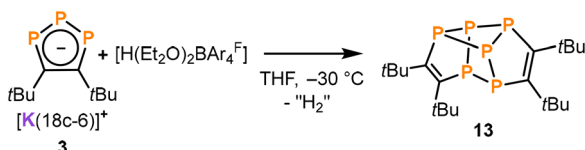
Scheme 3 Synthesis of 13 .
