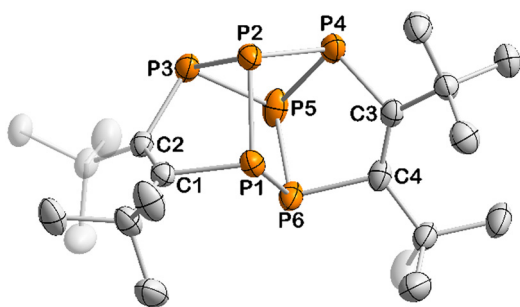
Fig. 5 Solid-state molecular structure of 13 . Displacement ellipsoids are drawn at the 50% probability level; H atoms have been omitted for clarity. Selected bond lengths (Å) and angles (°): P1–P2 2.1709(8), P1–P6 2.2380(8), P2–P3 2.2082(8), P2–P4 2.2571(8), P3–P5 2.2540(8), P4–P5 2.2054(9), P5–P6 2.1736(9), P1–C1 1.875(2), P3–C2 1.858(2), P4–C3 1.851(2), P6–C4 1.870(2), C1–C2 1.364(3), C3–C4 1.366(3), P1–P2–P3 90.50(3), C1–P1–P2 93.58(7), C2–P3–P2 99.04(7), C1–C2–P3 115.47(15), C2–C1–P1 116.22(15), P4–P5–P6 90.47(3), C3–P4–P5 98.78(7), C4–P6–P5 93.26(7), C3–C4–P6 115.92(15), C4–C3–P4 115.81(16), P1–P2–P4 87.60(3), P3–P2–P4 83.93(3), P4–P5–P3 84.07(3), P6–P5–P3 97.62(3).
