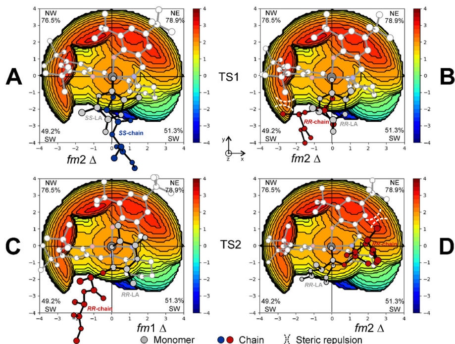
Fig. 7 % V_{\text{Bur}} steric maps of the RLS corresponding to TS1 for SS -LA (A) and RR -LA (B) propagations with catalyst ( R,R )- 2A . Steric interactions leading to the TS2 preference for fm1 (C) vs. fm2 (D) for RR -LA propagation are reported with dashed lines. The z-axis is perpendicular to the plane containing the map.
