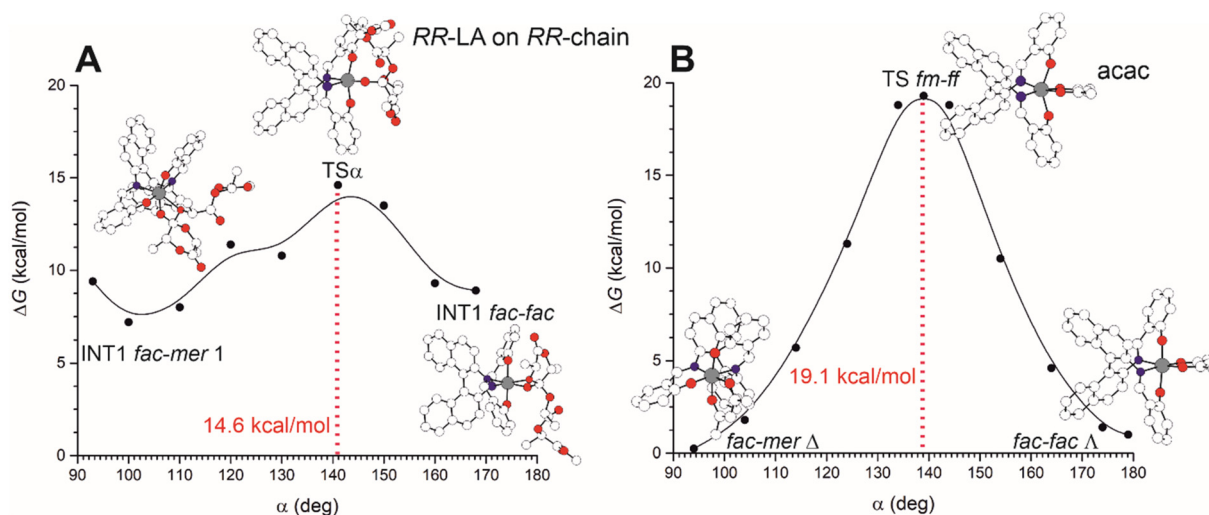
Fig. 4 Free energy profiles of the transformation from fac-mer \Delta to fac-fac \Delta for ( R )-1 as a function of the O_L-Al-O_L valence bond. The reorganization path moving from TS1 ( fm1 ) to TS2 ( ff ) as a function of \alpha for RR -LA polymerization is reported in A. The analogous path by using the bidentate acac − is reported in B. Aluminum, oxygen and nitrogen atoms in gray, red and blue. Hydrogen atoms have been omitted for clarity.
