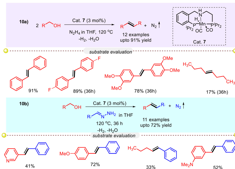
Scheme 10 Olefination of (10a) hydrazine and (10b) hydrazone via ADC strategy. 37
