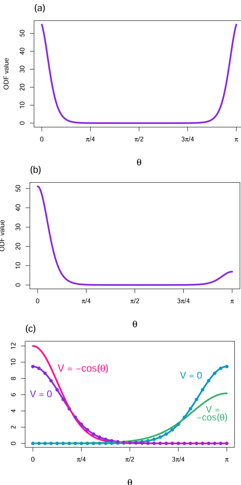
Fig. 8 ODF modulation by an external field. (a) Results for W(\gamma) = \sin(\gamma) with B = 12 , and an applied field V(\theta) = 2 \sin(\theta) which favors orientations around both \theta = 0 and \pi . The peak value of this ODF is even larger than that for the hard core reference system with B = 14 (cf. Fig. 2). (b) Results for W(\gamma) = \sin(\gamma) with B = 12 , and an applied field V(\theta) = -\cos(\theta) which favors orientations around \theta = 0 and disfavors orientations around \theta = \pi . (c) The pair of minima of the free energy for the dipolar kernel with V = 0 and B = 6 (purple and cyan) were obtained from initial values for the iteration having either a peak at \theta = 0 or a peak at \theta = \pi . The dots are exact values. 20 These ODFs are mirror images of each other about \pi/2 and are physically equivalent, since each can be obtained from the other by a rotation of spherical coordinates. In the presence of an applied field V(\theta) = -\cos(\theta) which favors orientation toward \theta = 0 , for starting values with a peak close to \theta = \pi the iteration converges to an ODF (green) that has attenuated orientation toward \theta = \pi . For other starting values, the iteration converges to an ODF (magenta) that has accentuated orientation toward \theta = 0 . The ODF with the accentuated peak at \theta = 0 has the lower free energy in the presence of the applied field.
