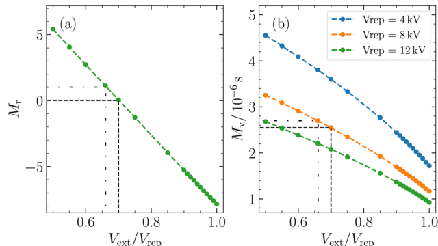
Fig. 2 Magnification of the positions M_r (a) and velocities M_v (b) is illustrated in the figure. These magnifications were calculated with SIMION for Na(MeOH) by mapping the position and velocities of the clusters at ionization and detection. The extractor voltage was swept while keeping the repeller voltage constant. The curves for three different repeller voltages are displayed. The black dotted line at V_{\text{ext}}/V_{\text{rep}} = 0.66 represents the ratio where a magnification of M_r = 1 is achieved, whereas the black dashed line at V_{\text{ext}}/V_{\text{rep}} = 0.7 represents VMI conditions ( M_r = 0 ).
