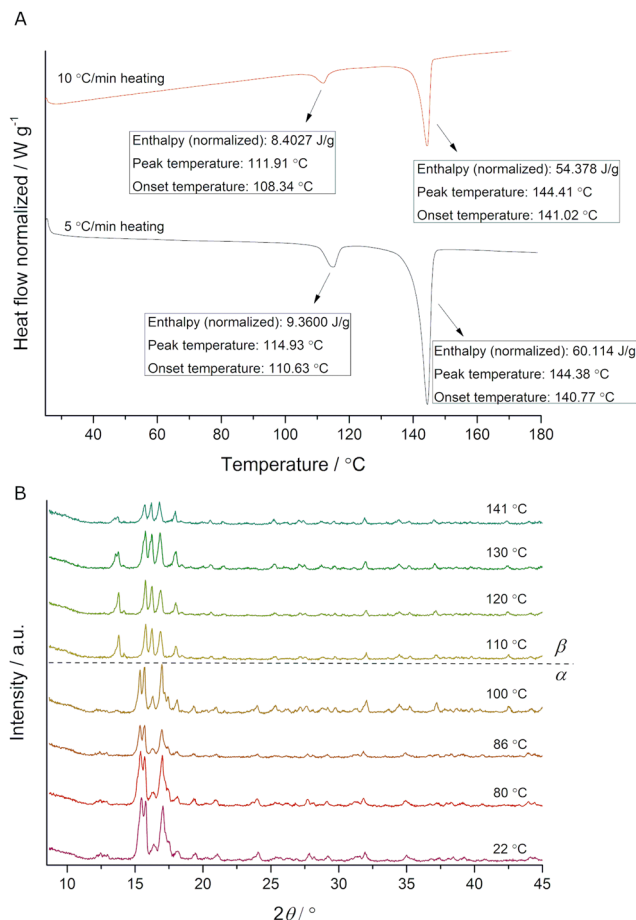
Fig. 2 (A) DSC traces of ADE obtained by applying different heating rates. Endotherms are pointing downwards. (B) In situ monitoring of ADE phase transition by VT-PXRD ( \lambda = 1.54 Å).
