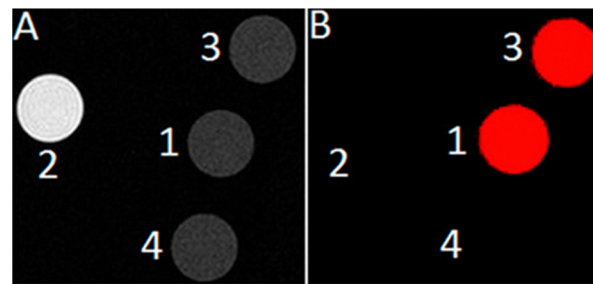
Fig. 6 Image (A) is a T_1 -weighted image, and image (B) is a CEST difference image. For both (A) and (B), spot 1 represents \text{Eu}^{\text{II}}\mathbf{8} , spot 2 represents \text{Eu}^{\text{II}}\mathbf{8} , spot 3 represents \text{Eu}^{\text{III}}\mathbf{8} from the oxidation of \text{Eu}^{\text{II}}\mathbf{8} , and spot 4 represents water. Reprinted with permission from L. A. Ekanger, D. R. Mills, M. M. Ali, L. A. Polin, Y. Shen, E. M. Haacke and M. J. Allen, Inorg. Chem. , 2016, 55 , 9981. Copyright 2016 American Chemical Society.
