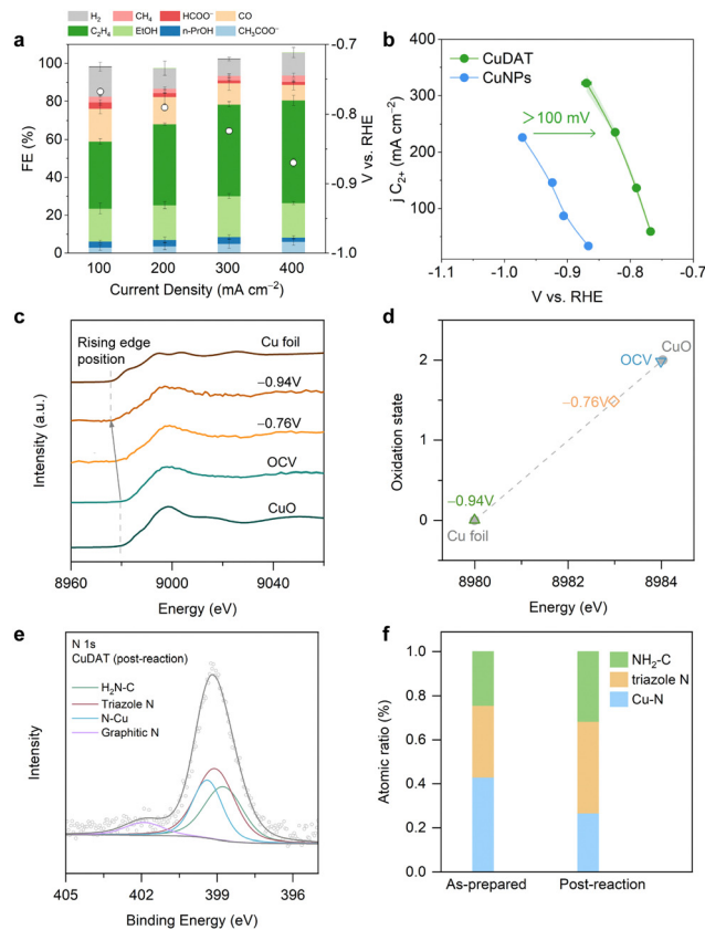
Fig. 2 (a) CO 2 R performance on CuDAT in 1 M KHCO 3 . (b) j_{\text{C}_{2+}} on the function of the overpotential for CuDAT and CuNPs. (c) Operando Cu K-edge XANES for CuDAT during CO 2 R in a flow cell. (d) Oxidation state, deduced from the rising edge energy of Cu K edge XANES in CuDAT during CO 2 R at different overpotentials. (e) N 1s XPS of the post-CO 2 R CuDAT and (f) atomic percentage of N species for as prepared and post-reaction CuDAT. Triazole N and amino N were largely reserved.
