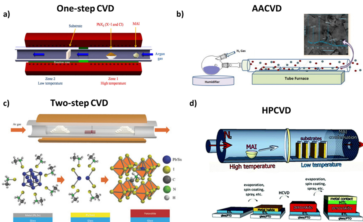
Fig. 7 (a) Schematics of the perovskite film fabrication using MAI and PbX_2 sources deposited onto a c-TiO_2 -coated FTO glass substrate which is performed in a CVD furnace. Adapted with permission from ref. 111. (b) Schematics of the all-inorganic perovskite CsPbBr_2 by an aerosol assisted CVD method. Adapted with permission from ref. 116. (c) Schematic of the CVD furnace and growth conditions of a perovskite film, and schematics of reaction details of the metal film with MAI, resulting in perovskite film formation. Adapted with permission from ref. 118. (d) Hybrid chemical vapor deposition based perovskite synthesis (top) diagram of the HPCVD furnace and MAI deposition onto metal halide seeded substrates. (Bottom) Layered structure of a complete solar cell fabricated by a HPCVD process. The complete solar cell is a glass substrate followed by a FTO layer, an electron transport layer, a perovskite layer, a hole transport layer, and a top metal contact. Adapted with permission from ref. 120.
