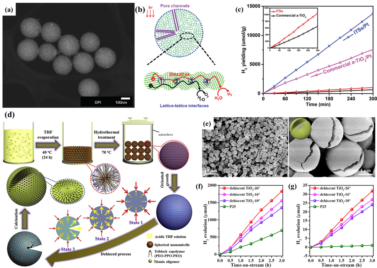
Fig. 10 (a) STEM image, (b) illustration of the charge transport, and (c) H 2 evolution of the integrated TiO 2 microspheres (ITSS). Reprinted with permission from ref. 103. Copyright © 2016, Wiley-VCH. (d) Schematic illustration of the synthesis and (e) SEM images with different magnifications of the dehiscent mesoporous TiO 2 microspheres. Water-splitting H 2 production by the dehiscent mesoporous TiO 2 microspheres with different crevice angles under (f) solar light and (g) visible light (> 400 nm). Reprinted with permission from ref. 108. Copyright © 2018, Elsevier Inc.
