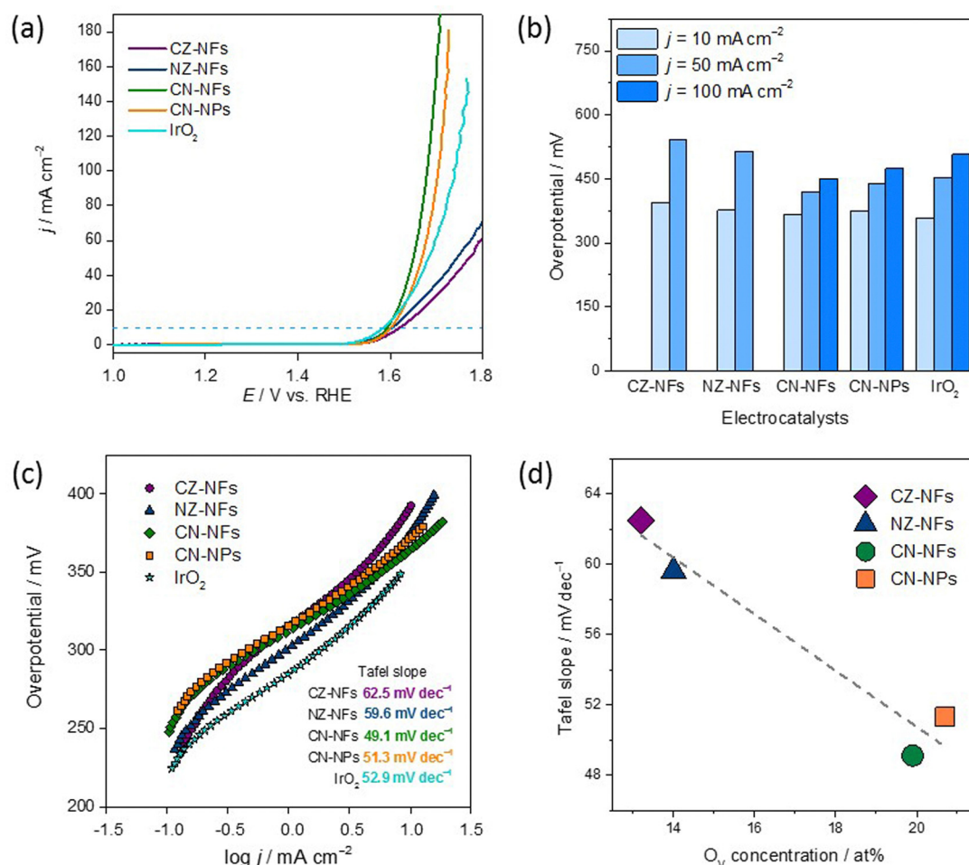
Fig. 5 (a) Linear sweep voltammograms of the spinel-type high-entropy oxides (CZ-NFs, NZ-NFs, CN-NFs, and CN-NPs) and \text{IrO}_2 reference material during OER in \text{O}_2 -saturated 1 M KOH, the dashed line highlights the values for the overpotential at 10 \text{ mA cm}^{-2} . (b) Comparison of the OER overpotentials at different current densities. (c) Tafel slopes of the considered electrocatalysts. (d) Tafel slopes of the HEOs as a function of the \text{O}_2 -concentration (a line is drawn to guide the eye).
