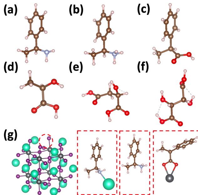
Fig. 1 Chiral molecules studied: (a) ( R )-methylbenzylamine ( R -MBA-H), (b) ( R )-methylbenzylammonium ( R -MBAmH + -H), (c) ( R )-methylphenyl acetate ( R -MPAC − -H), (d) ( S )-lactic acid, (e) ( S )-malic acid, and (f) ( S )-tartaric acid. (g) Illustration of binding configurations of chiral molecules considered to CsPbI 3 perovskite cluster surface. ( R )-MBA-H can bind to surface Cs + cations, ( R )-MBAmH + -H can substitutionally replace surface Cs + cations, and the deprotonated ( R )-MPAC − -H can bind to Pb ions which can substitutionally replace surface Cs + cations. The lactic acid series molecules can bind in a similar way as ( R )-MPAC − -H. The ions have the following color labeling: Pb (grey), I (purple), Cs (teal), C (brown), N (blue), O (red), H (white).
