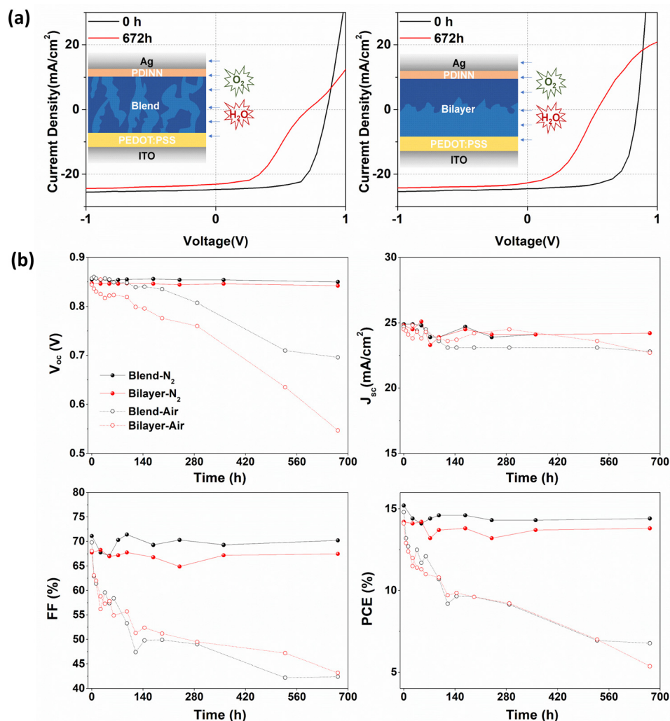
Fig. 4 (a) Scheme of water and \text{O}_2 diffusion into the OSC, and the corresponding J-V curves with blended and bilayer PALs stored in air. (b) Performance evolution of OSCs with blended (black curve) and bilayer (red curve) PALs stored in a glovebox ( \text{N}_2 – solid curve) and fume hood (air – dashed curve) for 672 hours.
