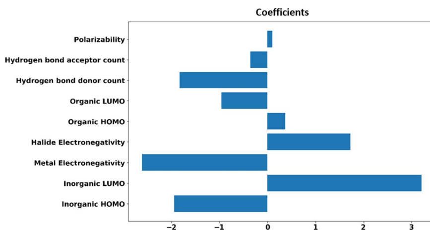
Fig. 5 Feature contributions of the finally selected nine features towards output Y.
