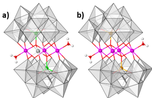
Fig. 7 Polyhedral representation of (a) [Co II (H 2 O) 2 Co II W VI (B- \alpha -Co II W 9 O 34 ) 2 ] 12- (Co 3 W-WS) and (b) [Co II (H 2 O) 2 Co II (B- \alpha -PW 9 O 34 ) 2 ] 10- (Co 4 -WS). Colour code: pink: Co II in octahedral geometry; green: Co II in tetrahedral geometry; grey: W; orange: P; red: O; white: H; grey polyhedra: {WO 6 } units. Note that the internal belt positions of Co 3 W-WS have a 50 : 50 Co : W equal occupancy.
