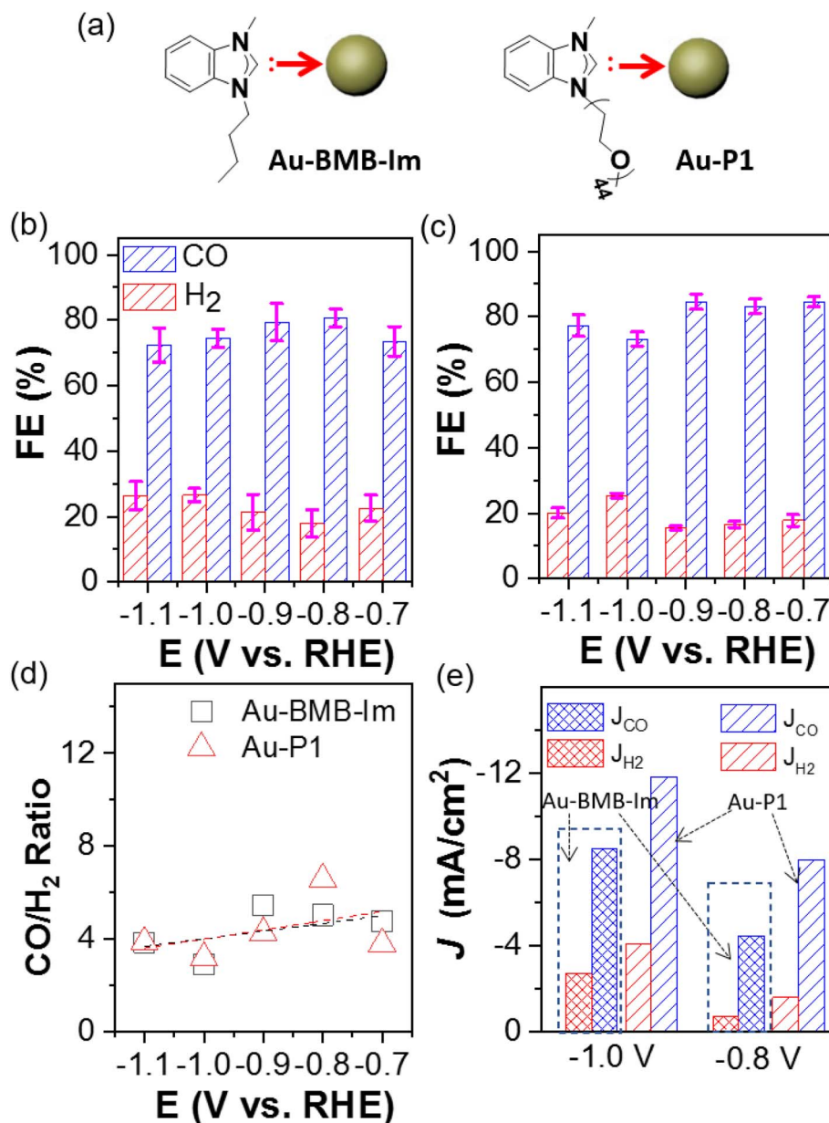
Fig. 3 (a) Scheme of BMB-Im and PEO-NHC modified AuNPs through Au-C binding. Catalytic selectivity to CO and H 2 using Au-BMB-Im (b) and Au-P1 (c). (d) Product ratio and (e) current density analysis of Au-BMB-Im and Au-P1.
