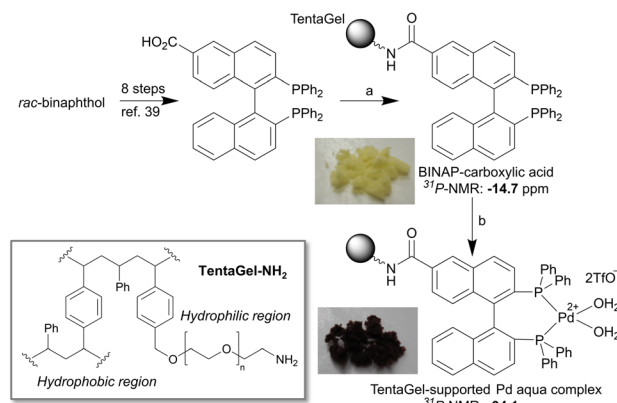
Scheme 1 Reagents and conditions: (a) TentaGel-NH 2 , EDCI, HOBT, DMF, retention time of 13 h. (b) [Pd(CH 3 CN) 4 ] 2+ (TfO − ) 2 , wet acetone, retention time of 7 h, 96% in 2 steps.
